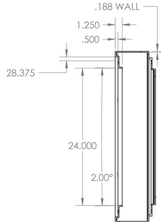
SECTION E-E
